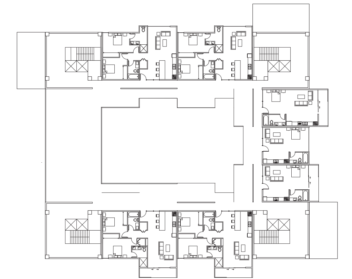
Floor Plan 1/32" = 100'
